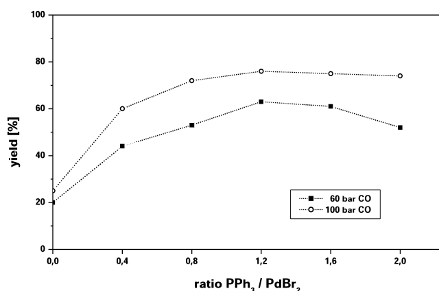
Figure 8. Influence of ligand to metal ratio: reactions were run in the six-fold parallel autoclave for 12 h at 100 °C using 15 mL NMP (1 M in acetamide and 2 M in propionaldehyde) and 0.25 mol % PdBr 2 , PPh 3 , 10 mol % LiBr, 1.5 mol % H 2 SO 4 .
