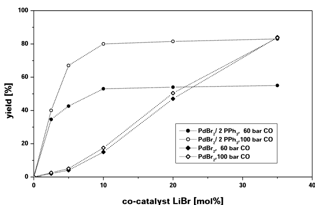
Figure 5. Influence of co-catalyst LiBr: reactions were run in the six-fold parallel autoclave for 12 h at 100 °C using 15 mL NMP (1 M in acetamide and 2 M in propionaldehyde) and 0.25 mol % catalyst, 1.5 mol % \text{H}_2\text{SO}_4 .
