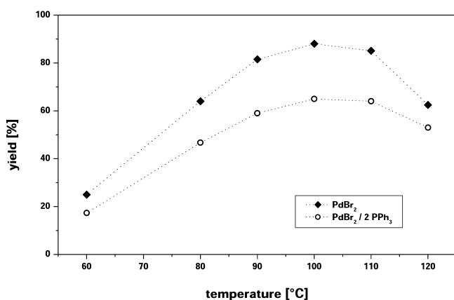
Figure 3. Influence of temperature: reactions were run for 12 h at 60 bar CO pressure using 50 mL NMP (1 M in acetamide and 2 M in propionaldehyde), 0.25 mol % catalyst, 35 mol % LiBr, 1.5 mol % H 2 SO 4 .
