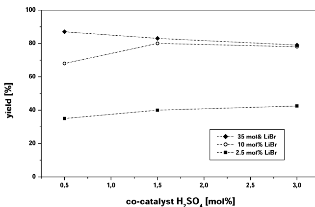
Figure 7. Determining synergistic effects of co-catalysts LiBr and \text{H}_2\text{SO}_4 : reactions were run in the six-fold parallel autoclave for 12 h at 60 bar CO pressure using 15 mL NMP (1 M in acetamide and 2 M in propionaldehyde) and 0.25 mol % \text{PdBr}_2/2 \text{PPh}_3 .
