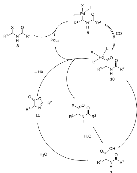
Scheme 4. Proposed mechanism for the palladium-catalyzed carbonylation.
