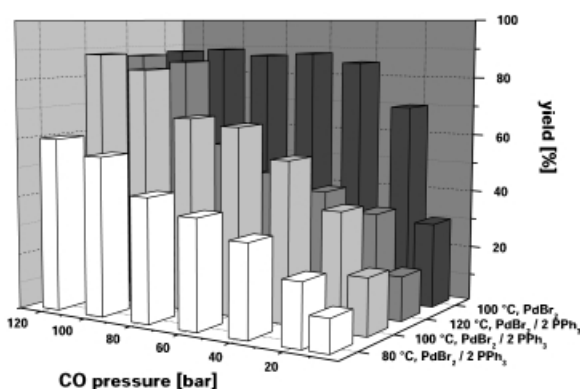
Figure 4. Influence of temperature and pressure: reactions were run for 12 h at 60 bar CO pressure using 50 mL NMP (1 M in acetamide and 2 M in propionaldehyde) and 0.25 mol % catalyst, 35 mol % LiBr, 1.5 mol % H 2 SO 4 .
