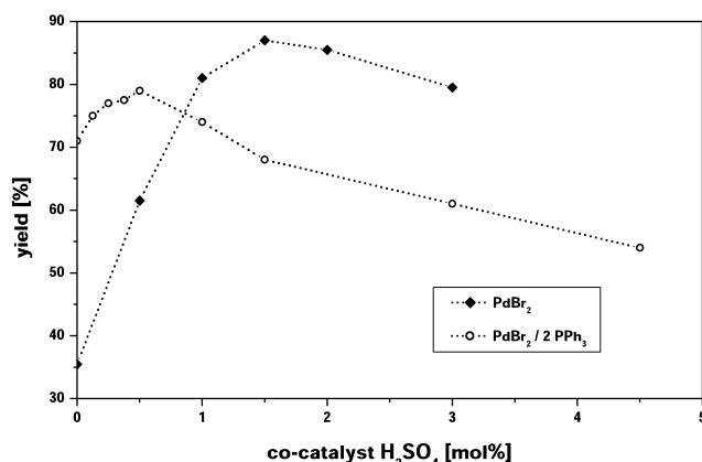
Figure 6. Influence of co-catalyst \text{H}_2\text{SO}_4 : reactions were run for 12 h at 60 bar CO pressure and 100 °C using 50 mL NMP (1 M in acetamide and 2 M in propionaldehyde) and 0.25 mol % catalyst, 35 mol % LiBr.
