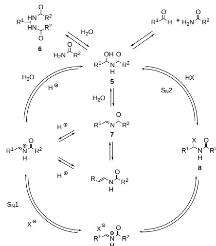
Scheme 3. Proposed pre-equilibria for the Pd-catalyzed amidocarbonylation.
