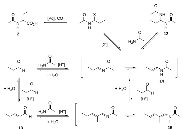
Scheme 5. Major equilibrating species in propionaldehyde-acetamide condensation reactions and palladium-catalyzed amidocarbonylation reaction.
